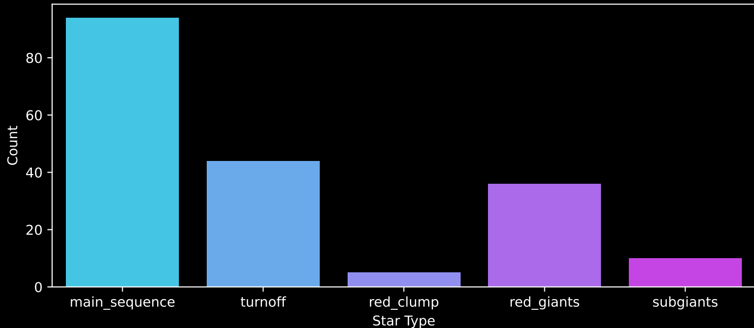
APOGEE DR17 Field: [177+51_MGA] Count plot of Star Type
