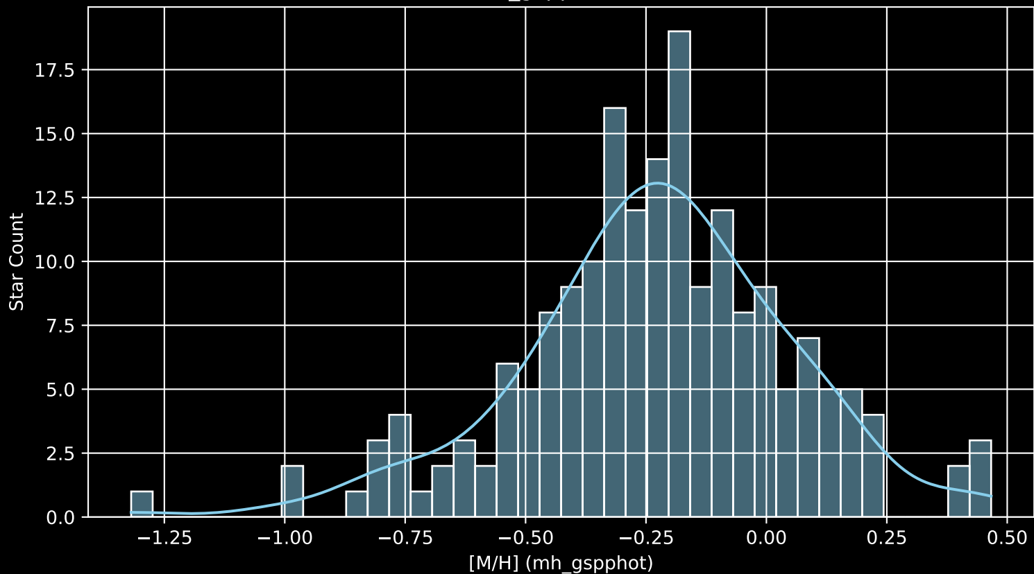
APOGEE DR17 Field: [177+51_MGA [M/H] (mh_gspphot) (n= 187)
