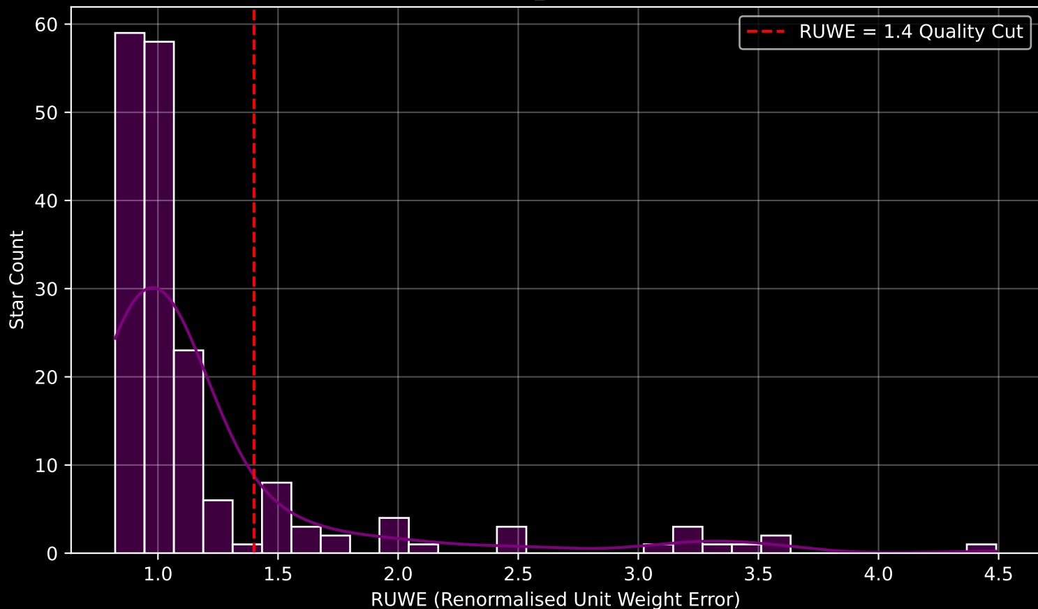
GAPOGEE DR17 Field [177+51_MGA] RUWE Distribution (n= 177)
