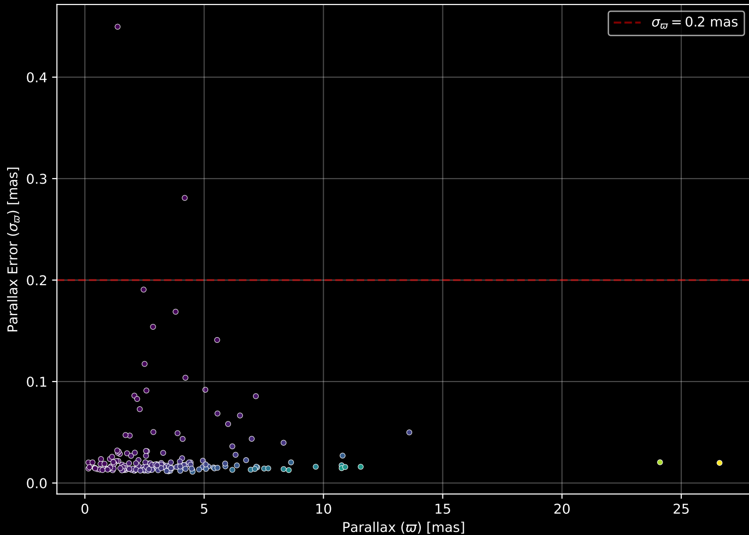
APOGEE DR17 Field: [177+51_MGA] Parallax Quality (n= 189)
