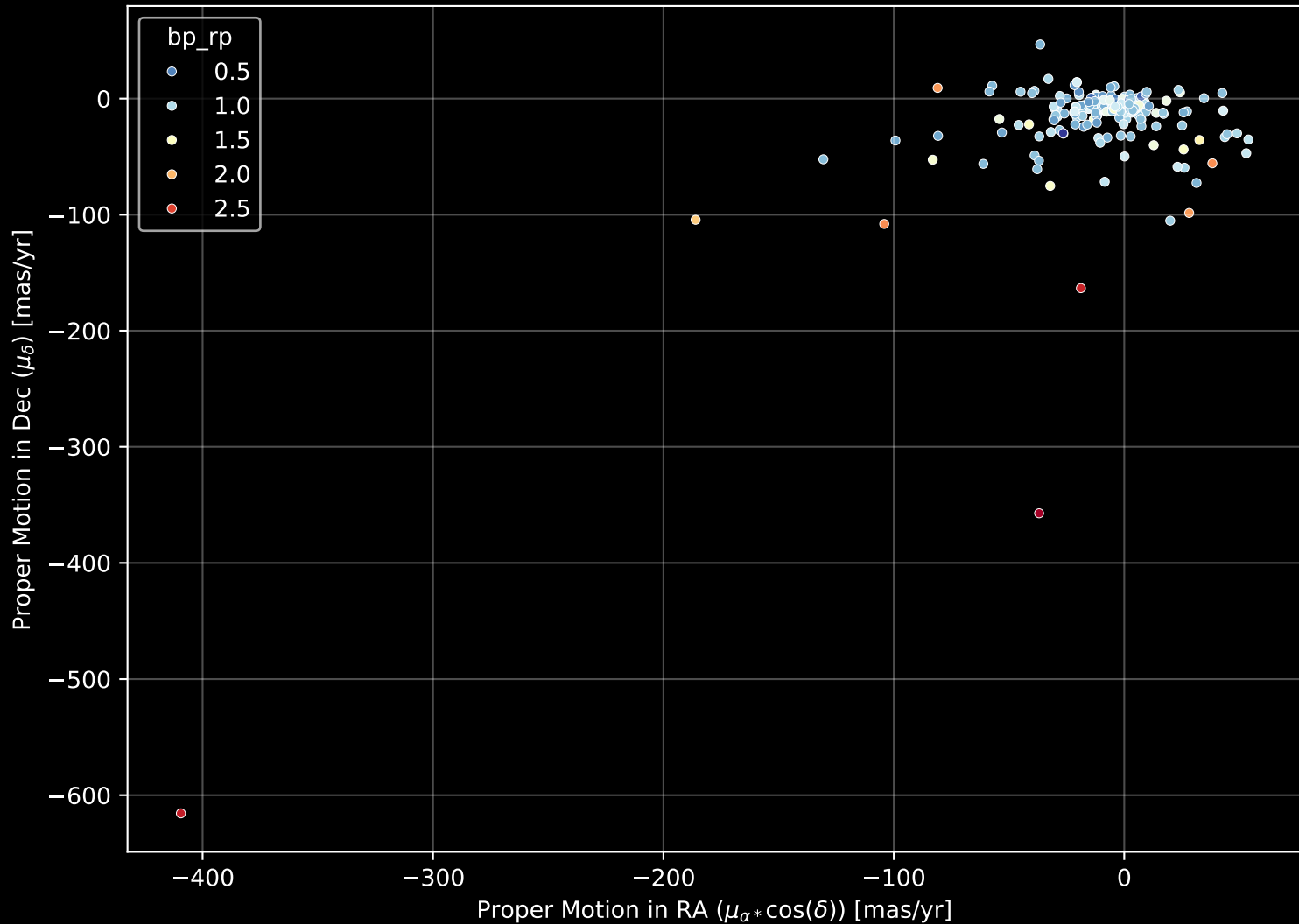
APOGEE DR17 Field: [177+51_MGA] Proper Motion Diagram (n= 189)
